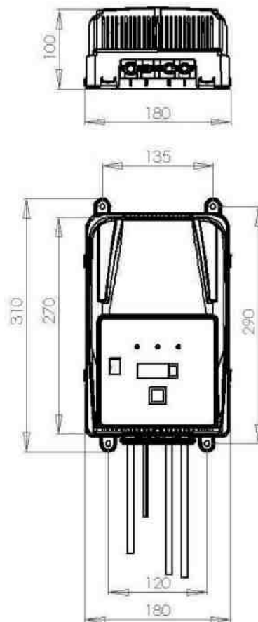
Dimensions in mm
